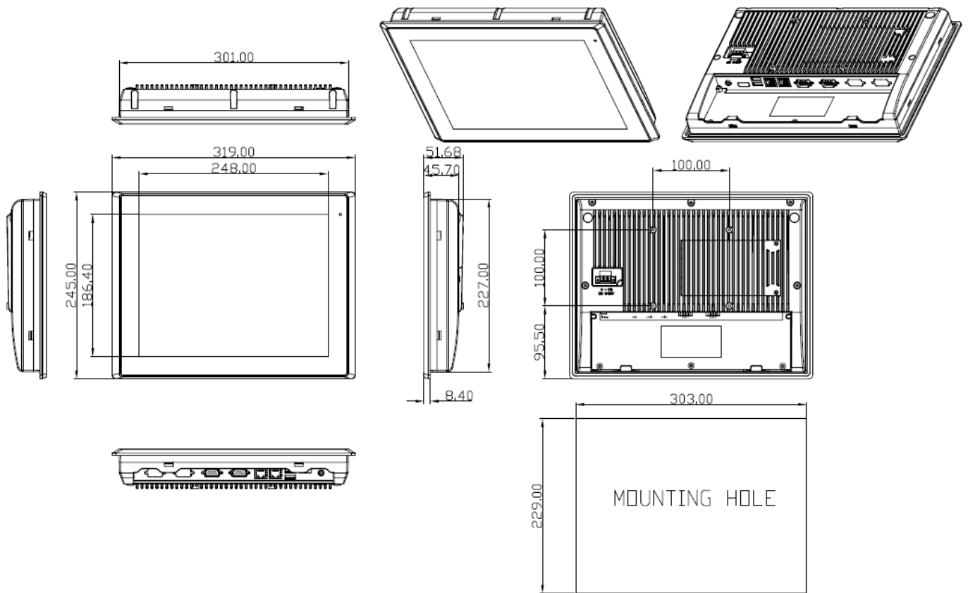
Figure 1.3: Dimensions of ARCHMI-712
